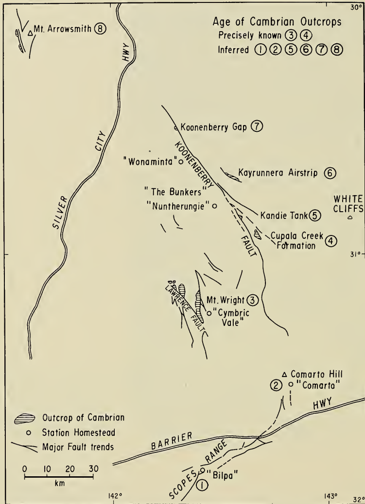
Fig. 8. Distribution of Cambrian strata in northwestern New South Wales.
